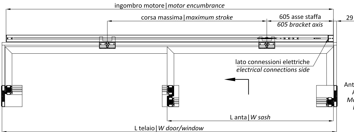
Schema | Type A
