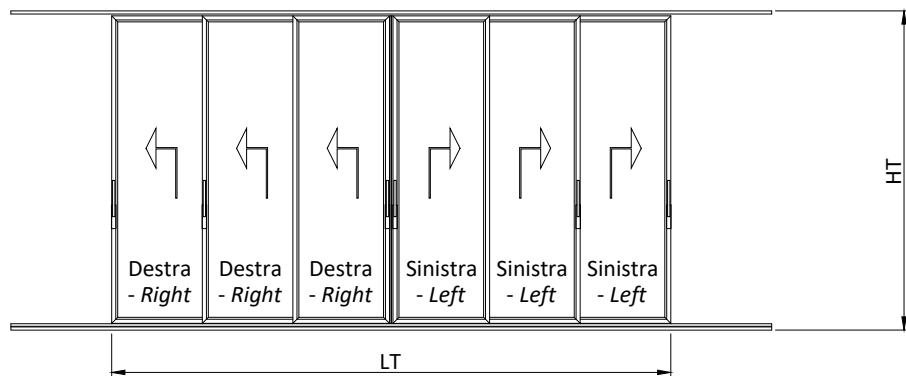
Schema | Type T3 6 ante scorrevoli coassiali a scomparsa 6 coaxial sliding sashes into the wall
