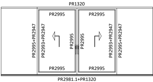
Schema | Type T1
